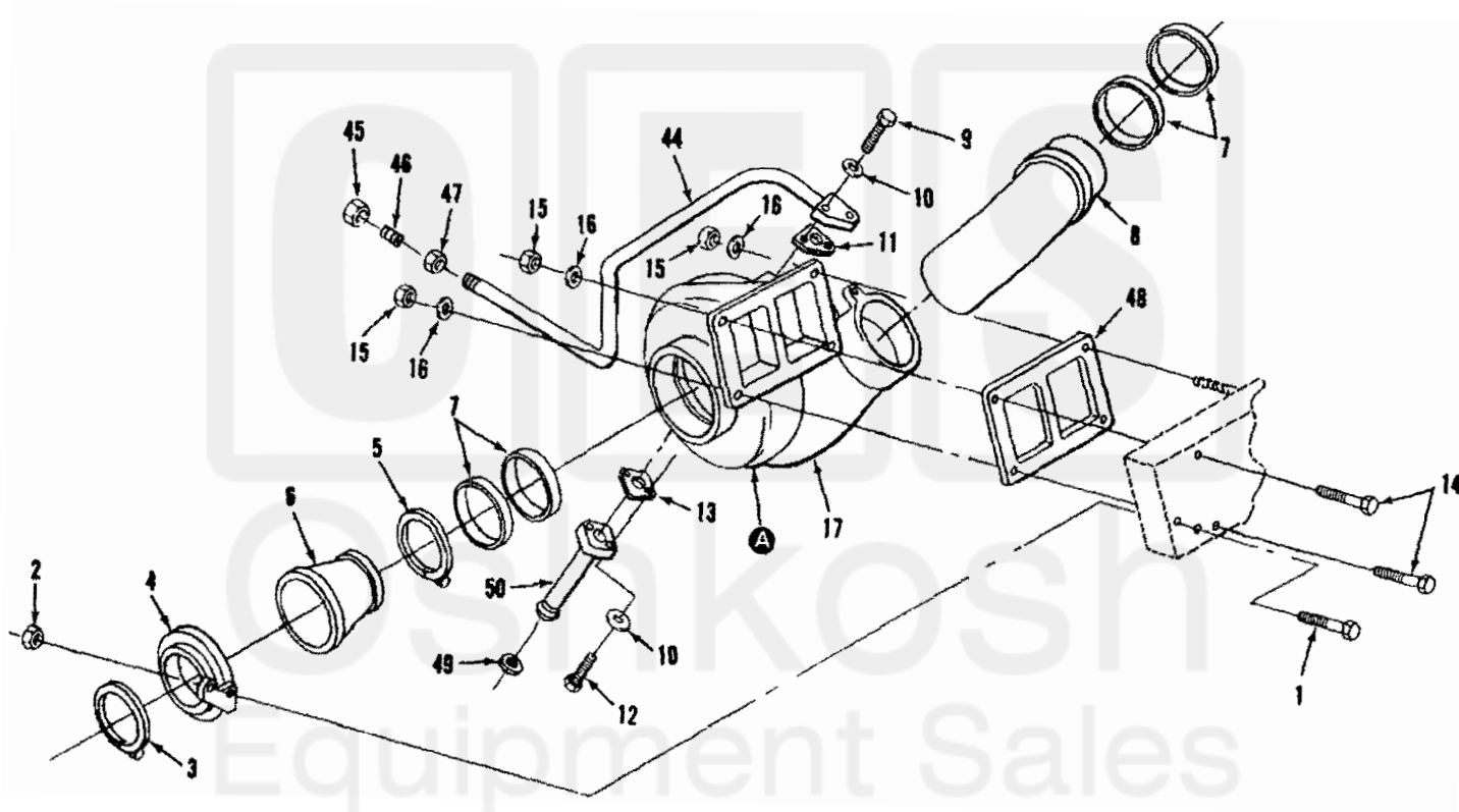
Figure 55. Turbocharger (Sheet 1 of 2)
